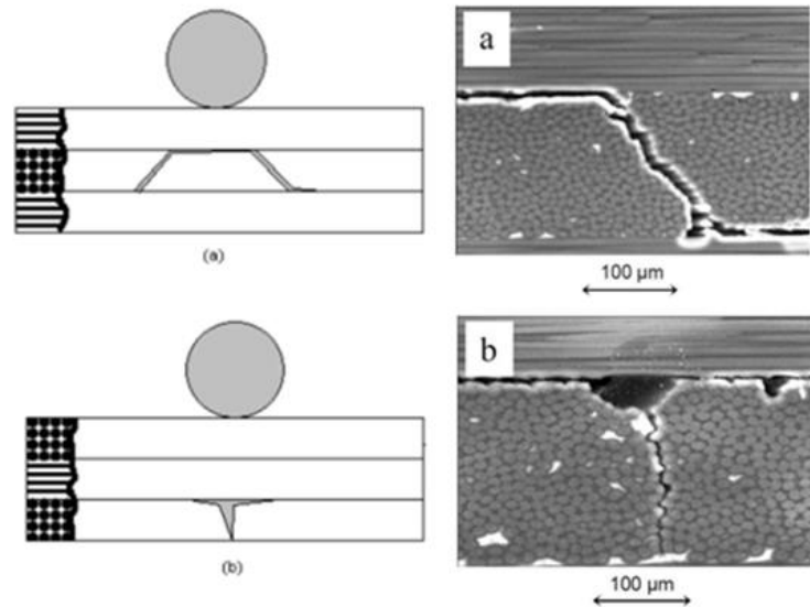
Figure 5 (a) tensile crack, (b) shear crack. [17, 26]
