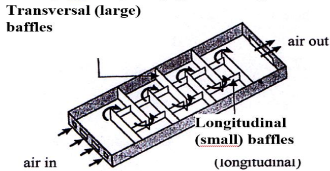
Figure 7 Solar panel equipped with TL type baffles
