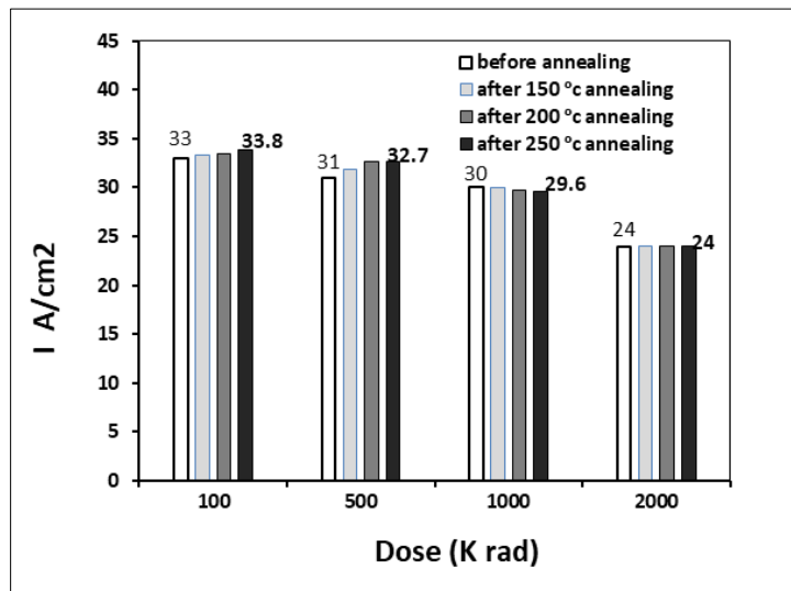
Figure 3 The recovery in solar cells short circuit current by thermal annealing
