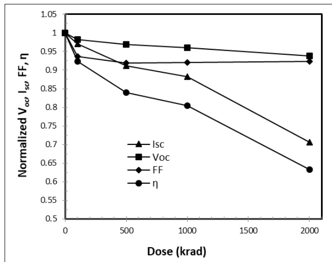
Figure 2 Normalized solar cell parameters as a function of gamma radiation dose
