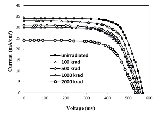
Figure 1 The I-V characteristics of silicon solar cell irradiated with various doses of gamma radiation
