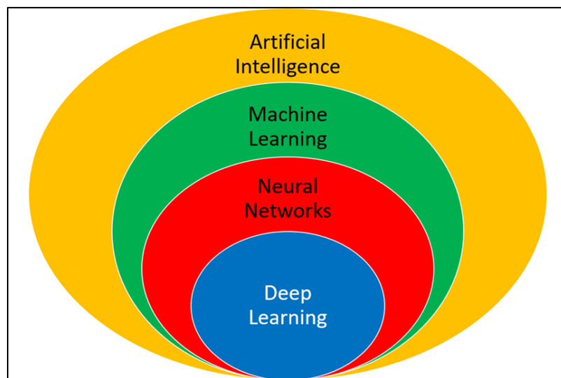
Figure 4 Deep Learning
