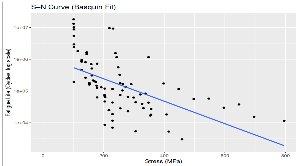
Figure 5: Stress–life (S–N) curve for the 7075-T651 aluminum alloy with a Basquin regression fit on \log_{10}(N_f) versus the applied stress amplitude.
