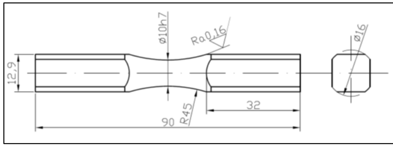
Figure 1: Geometry of the samples used in the experiments
