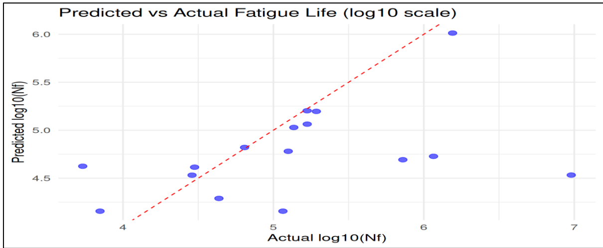
Figure 7: Predicted versus actual fatigue life (log10 scale)
